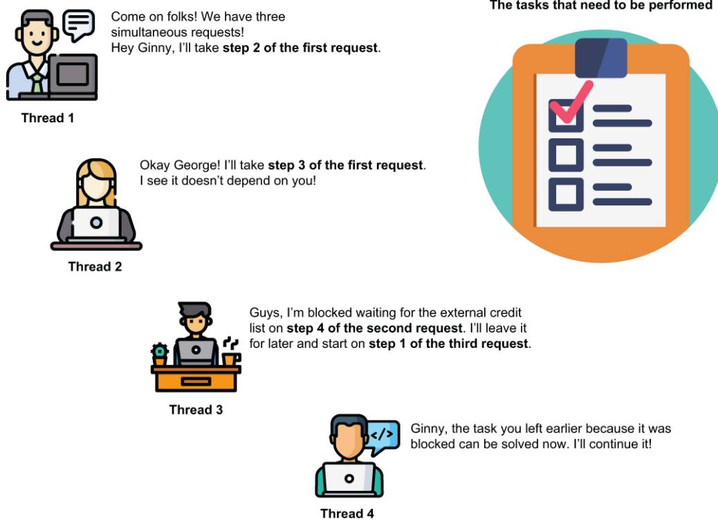
Figure 11.9 An analogy of the way a reactive app works. A thread doesn't take a request's tasks in order and wait when it's blocked. Instead, all tasks from all requests are on a backlog. Any available thread can work on tasks from any request. This way, independent tasks can be solved in parallel, and the threads don't stay idle.
