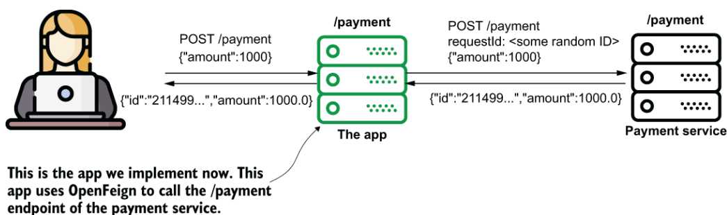
Figure 11.4 We now implement the app that consumes the /payment endpoint the payment service exposes. We use OpenFeign to implement the functionality that consumes the REST endpoint.
