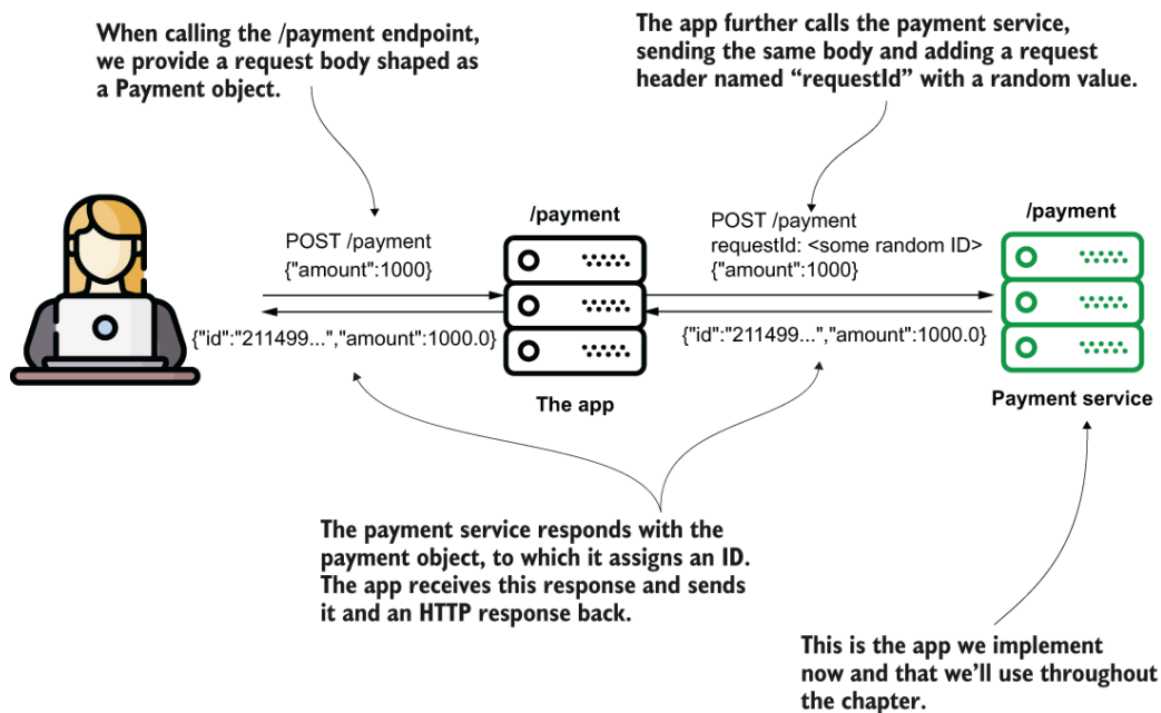
Figure 11.3 The payment service exposes an endpoint that requires an HTTP request body. The app uses OpenFeign, RestTemplate, Or WebClient to send requests to the endpoint the payment service exposes.
